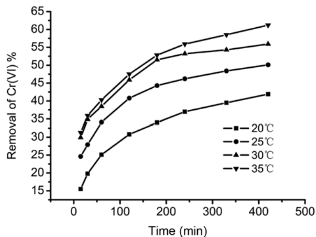
Fig. 3. Effect of temperature with time at concentration of 20 mg/L, \text{pH}=3.0 .
