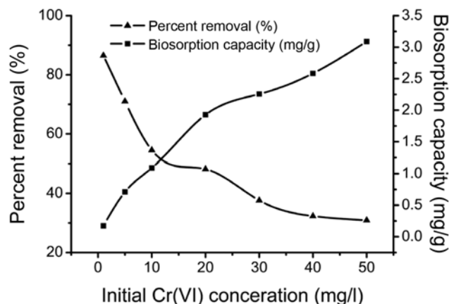
Fig. 2. Effect of initial concentration at T=30^\circ\text{C} , \text{pH}=3.0 .
