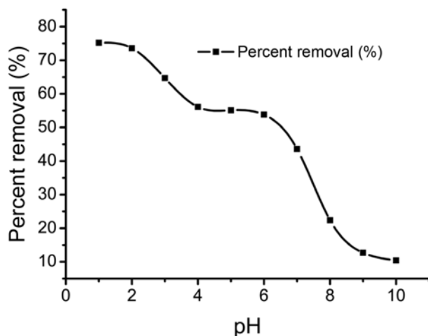
Fig. 1. Effect of initial pH on biosorption at concentration of 20 mg/L, T=30^\circ\text{C} .
